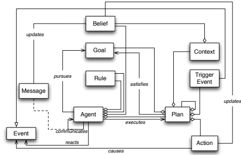
Figure 1. The Jason Metamodel
