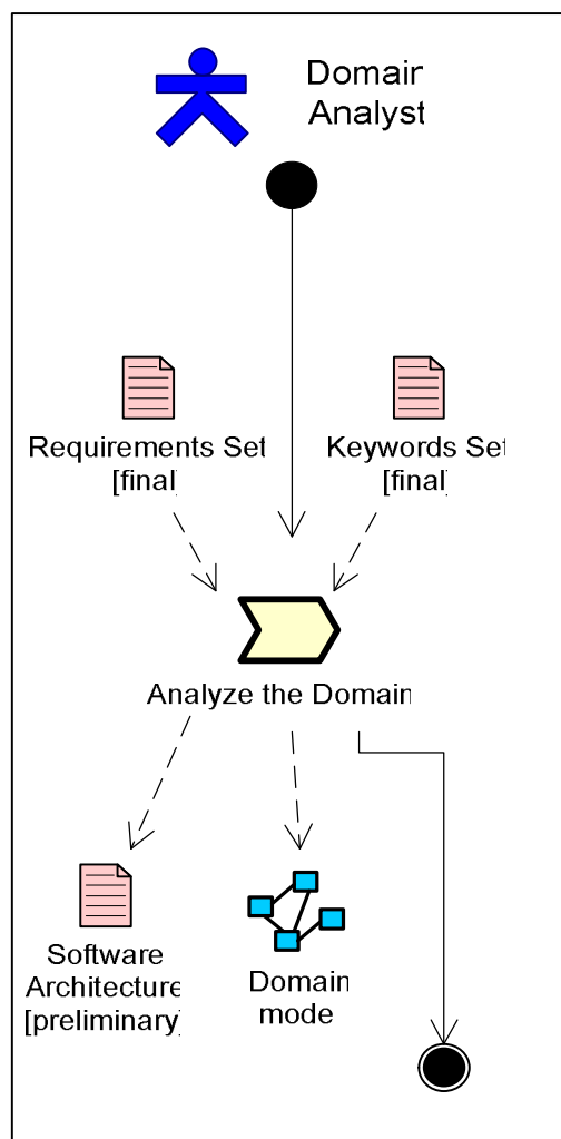
Figure 17. Domain Description
