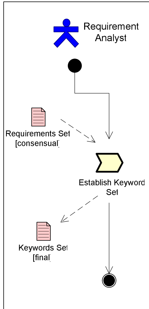
Figure 9. Keywords Identification
