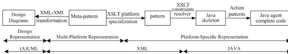
Fig. 2. The process used to obtain the platform specific pattern from its meta-representation
