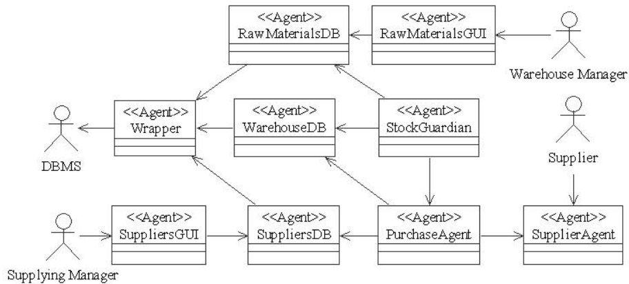
Fig. 4. A class diagram reporting the agents involved in the experiment and their relationships (communications)
