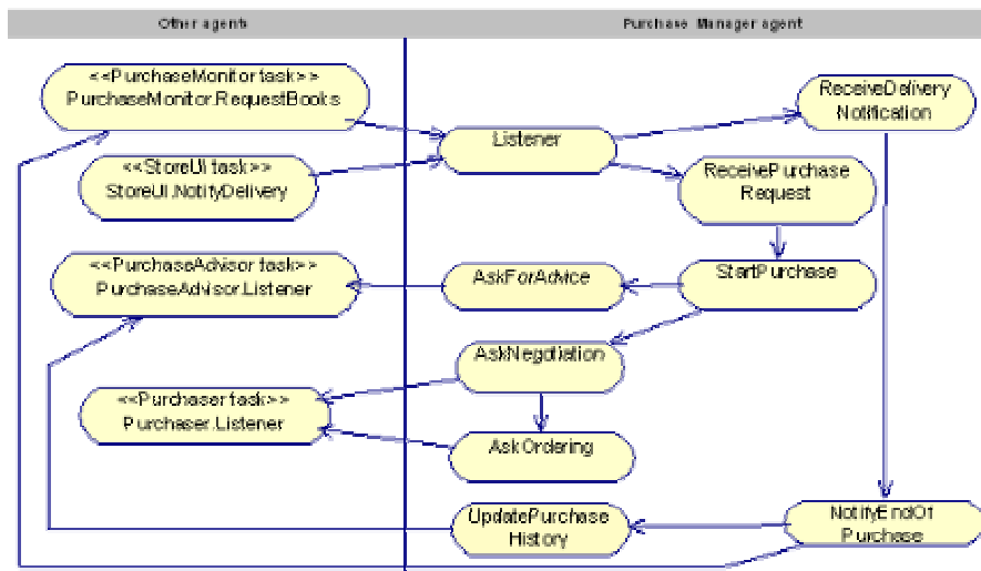
Fig. 4 The Task Specification Diagram
