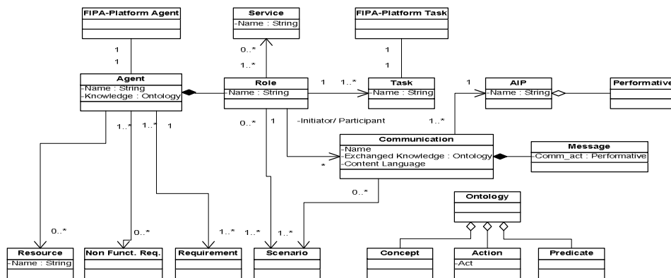
Fig5.. The MAS meta-model adopted in PASSI
