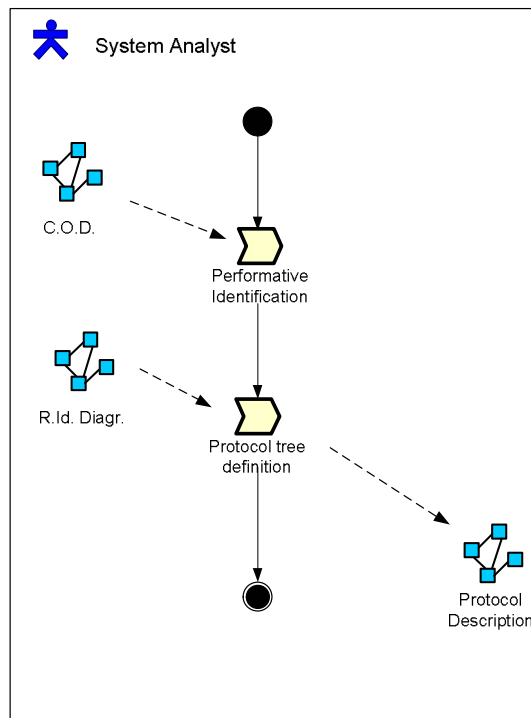
Fig.3 Protocols Description fragment-Procedural aspect
